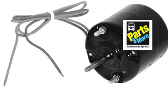
1075031 2 SPEED, CW, 1/4" SHAFT. IC #411876C1 BB #935494 THOMAS #85660130
