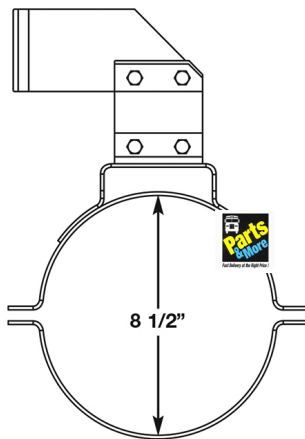
OE# CATALYTIC MUFFLER PART# TMVP1249 6224-1249
