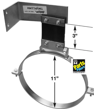
PART# TMVP11MH
