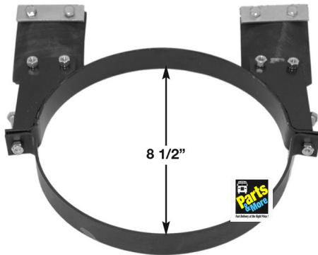
OE# MUFFLER HANGER PART# TP85MH 6224-0514 6224-0523
