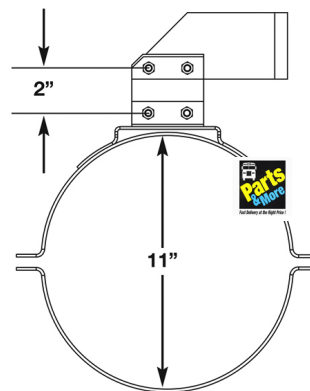
CATALYTIC MUFFLER PART# TMVP1250 6224-1250 OE#
