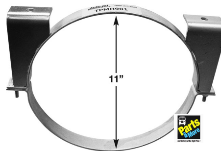
OE# MUFFLER HANGER PART# TPMH901 6224-0901 6224-0537 (BOTTOM)
