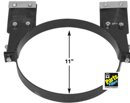
OE# MUFFLER HANGER PART# TP11MH 6224-0538 6224-0537 (BOTTOM)
