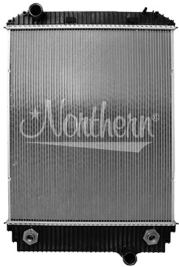
239085 RADIATOR FITS THOMAS & FREIGHTLINER 28 5/8" X 25" X 1 7/8"
